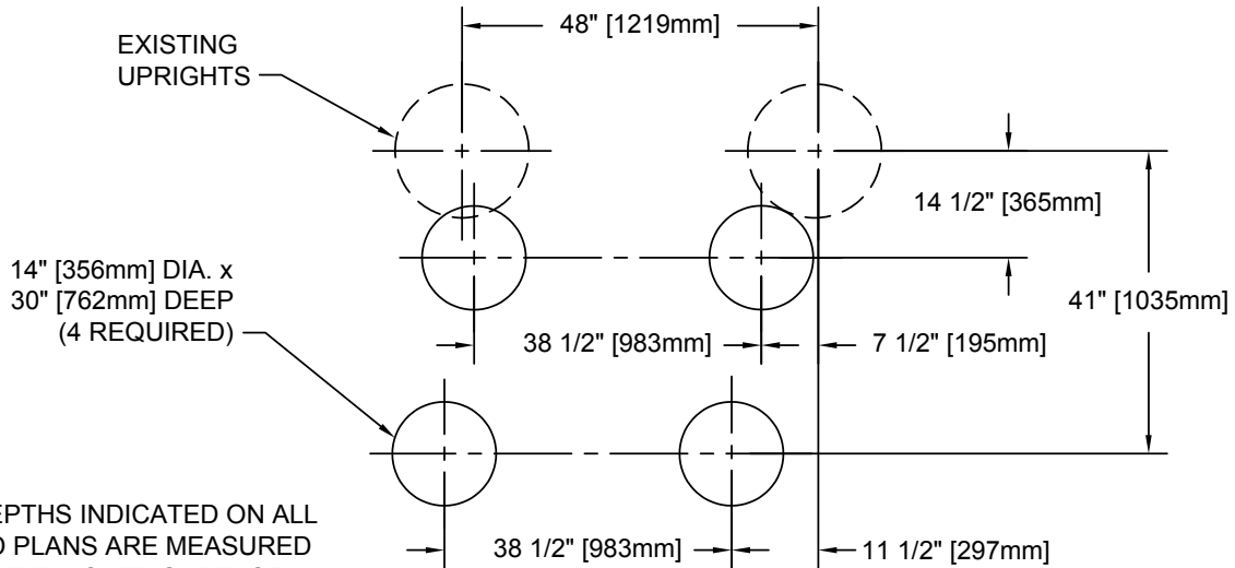
GROUND PLAN
