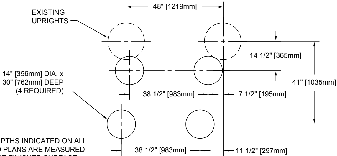
GROUND PLAN
