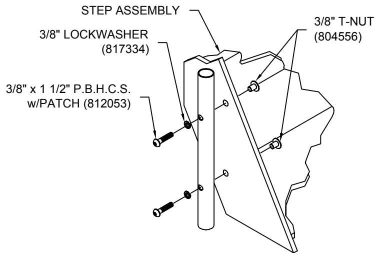
DETAIL "B"
