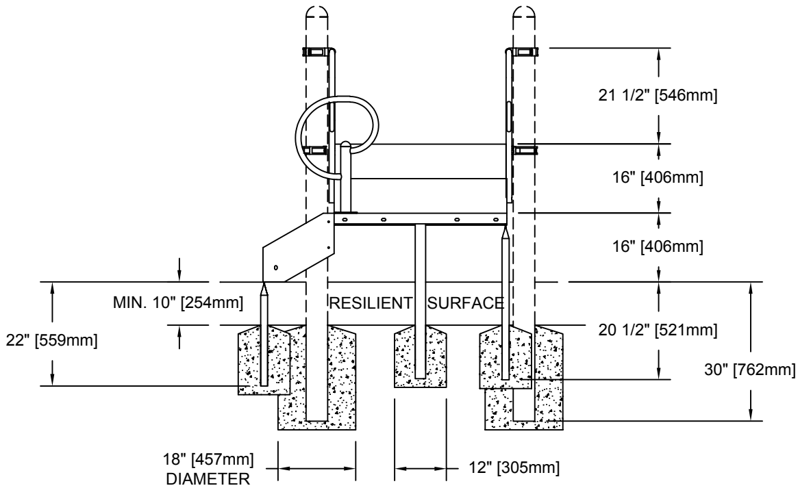
ELEVATION VIEW
