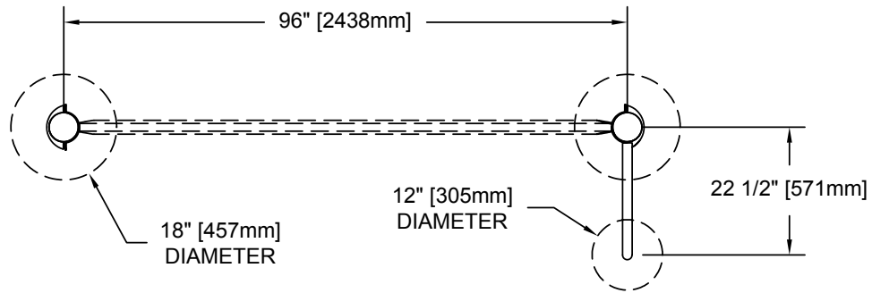
FOOTING DIAGRAM
