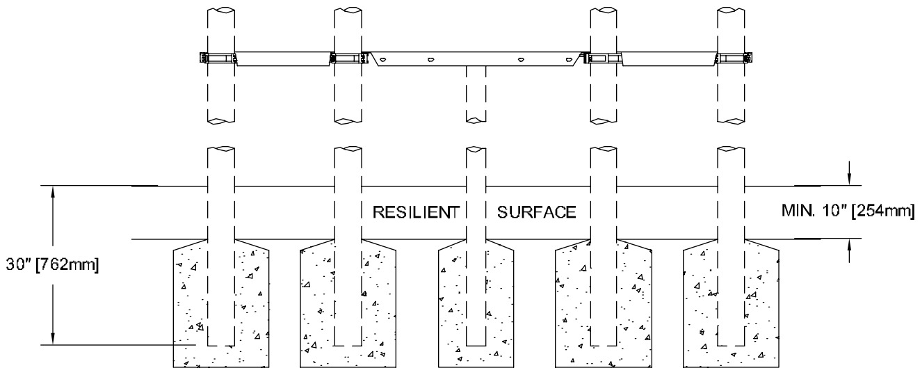
ELEVATION VIEW
