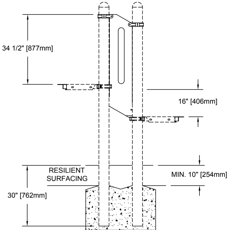
ELEVATION VIEW
